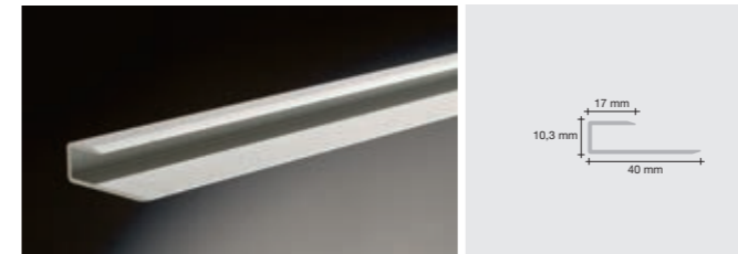
End moulding, silver PGENPCSILVME270, 2700 x 17 mm
