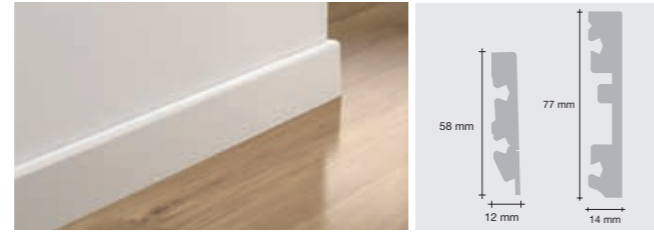
Wallbase, straight PGSKWHITE, 2400 x 12 x 58 mm – white* PGSKPAINT, 2400 x 12 x 58 mm – paintable* PGPSKWHITE, 2400 x 14 x 77 mm – white PGPSKPAINT, 2400 x 14 x 77 mm – paintable
