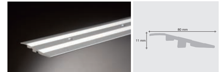
Ramp profile, silver PGRPC80SILVME270, 2700 x 80 mm
